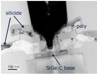
Fig2: TEM Cross section of Infineon's SA selective epitaxial base HBT
