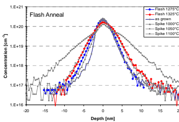
Fig 4: SIMS measurements of B profiles annealed at different temperatures with a conventional spike anneal (gray lines) or flash anneal (blue and red line)
