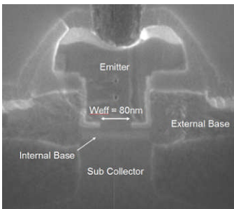
Fig 3: SEM cross-section of novel device
