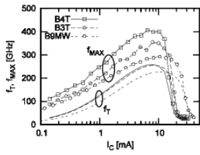
Fig1: f_T and f_{max} of STMicroelectronics's BiCMOS9MW, B3T and B4T technology
